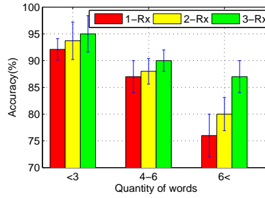
Figure 13: Performance with Multiple Rx.
